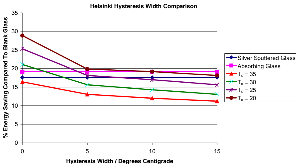
Figure 13. It shows the percentage energy saving of each system when compared to the blank glass system with variation of hysteresis width.
