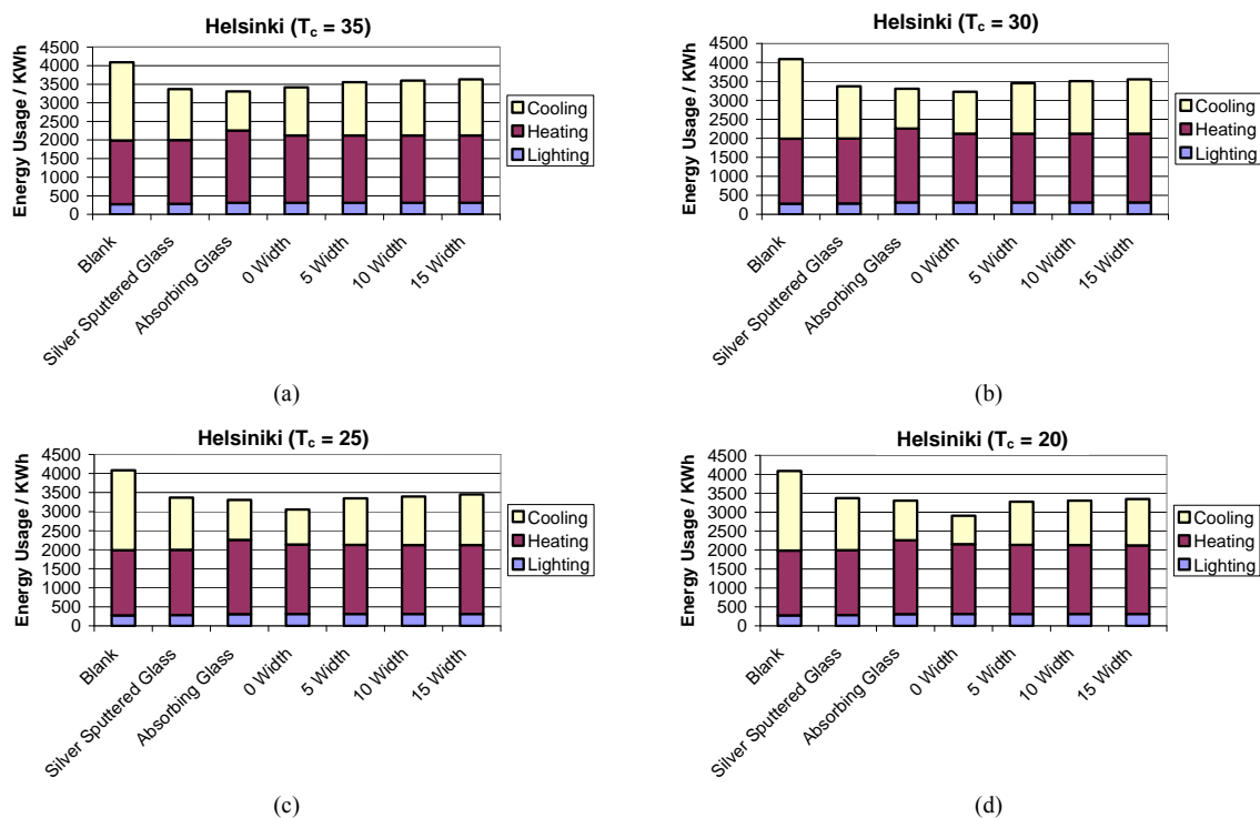
Figure 12. (a)-(d) show the breakdown of energy usage in a commercial building model based in Helsinki for varying values of T_c ((a) = 35^\circ\text{C} , (b) = 30^\circ\text{C} , (c) = 25^\circ\text{C} , (d) = 20^\circ\text{C} ) and varying hysteresis width ( 0^\circ\text{C} , 5^\circ\text{C} , 10^\circ\text{C} , 15^\circ\text{C} ). Each graph shows all modelled glazing systems. The colours correspond to the different energy requirements; yellow = cooling, maroon = heating, blue = lighting.
