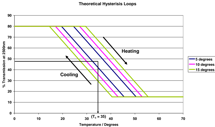
Figure 3. Diagram showing the theoretical hysteresis loops modelled for T_c = 35^\circ\text{C} .
