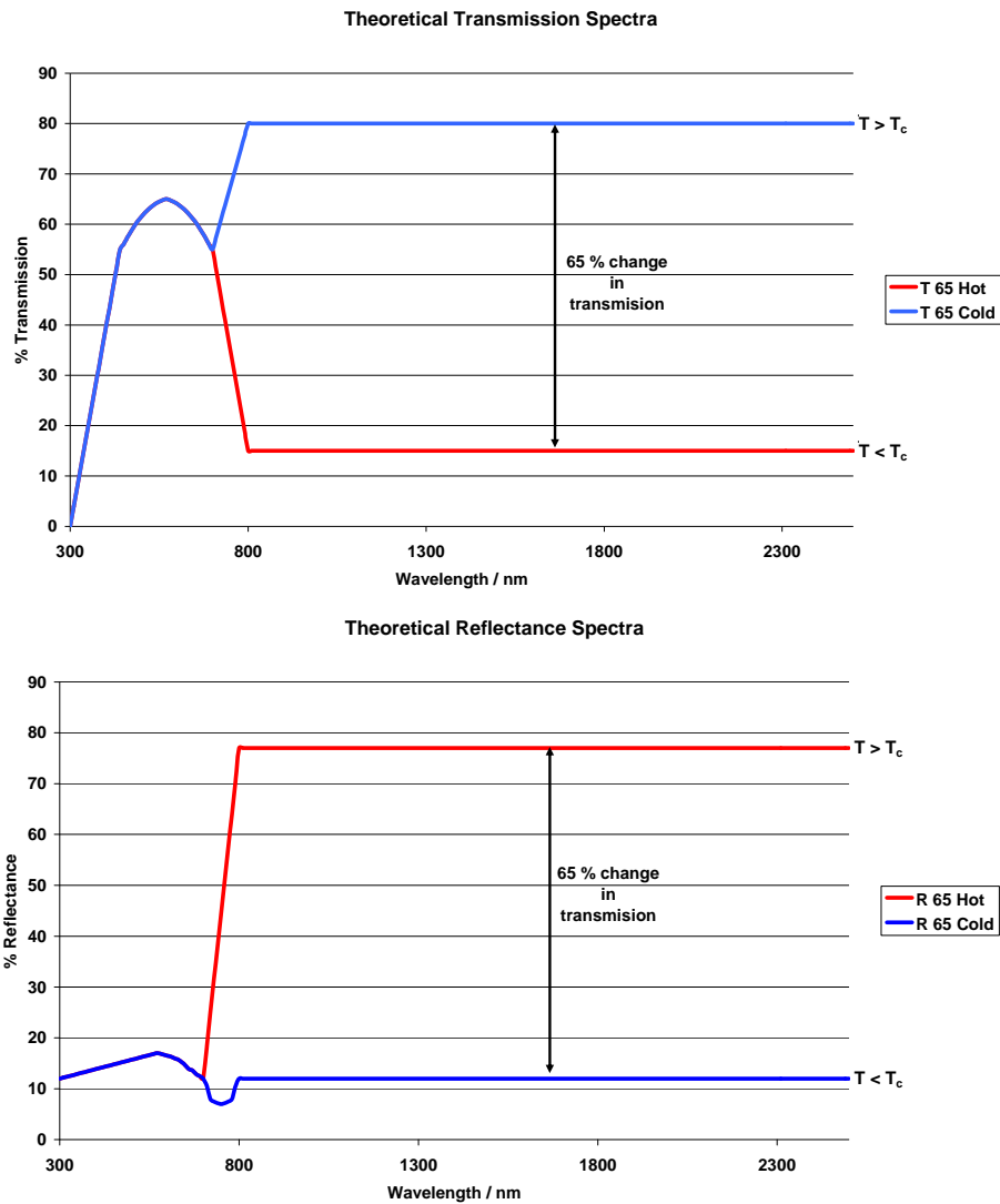
Figure 2. Theoretical transmission/reflectance data.
