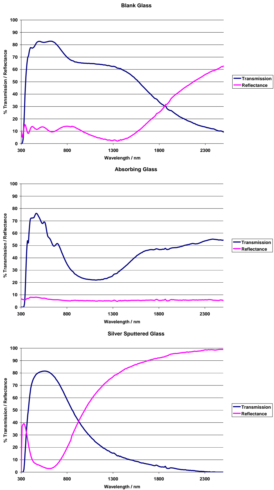
Figure 1. Transmission/reflectance spectral data for industrial standards and blank glass.
