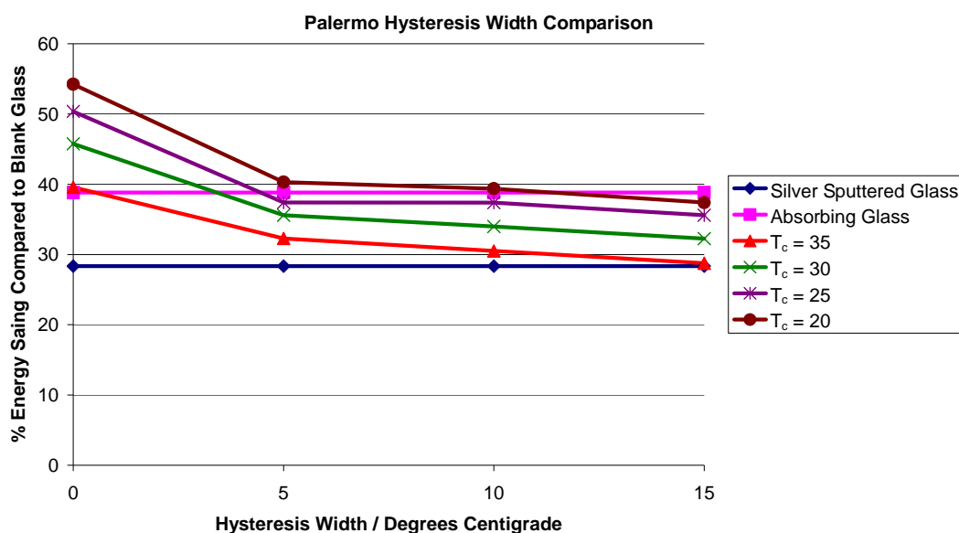
Figure 9. Shows the percentage energy saving of each system when compared to the blank glass system with variation of hysteresis width.
