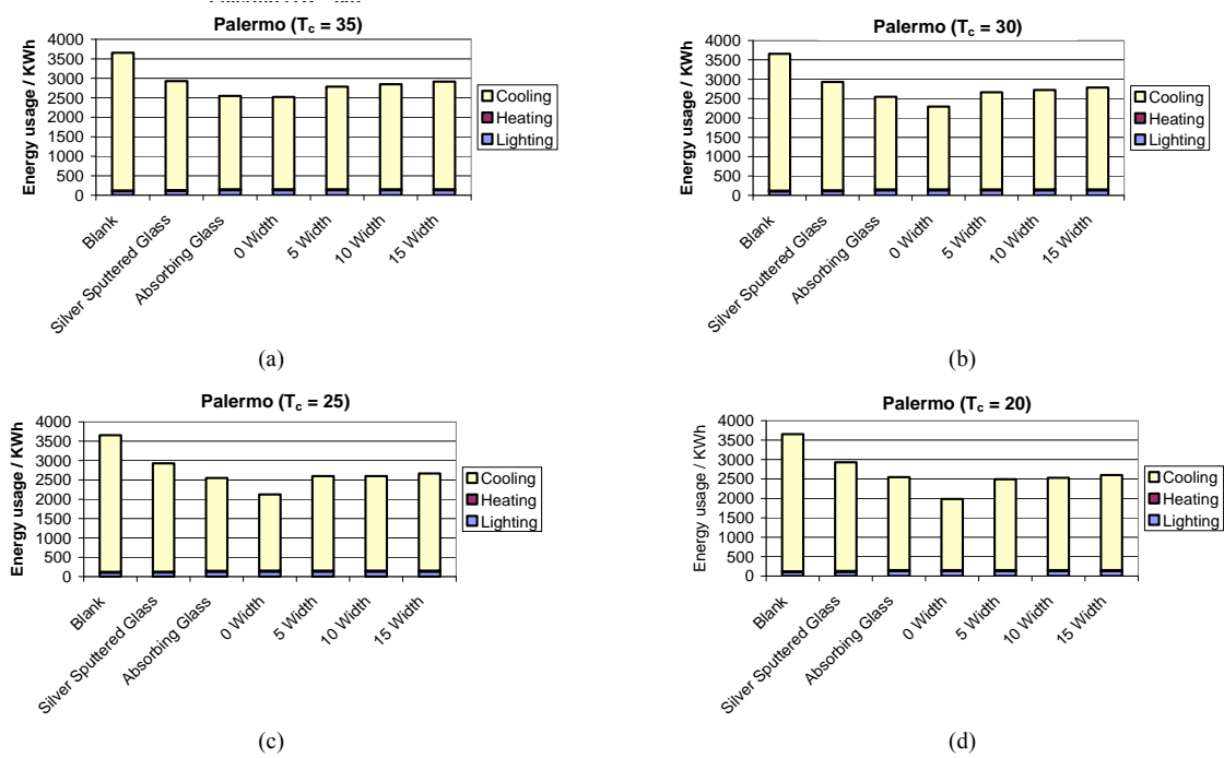
Figure 8. (a)-(d) show the breakdown of energy usage in a commercial building model based in Palermo for varying values of T_c ((a) = 35°C, (b) = 30°C, (c) = 25°C, (d) = 20°C) and varying hysteresis width (0°C, 5°C, 10°C, 15°C). Each Graph shows all modelled glazing systems. The colours correspond to the different energy requirements; yellow = cooling, maroon = heating and blue = lighting.
