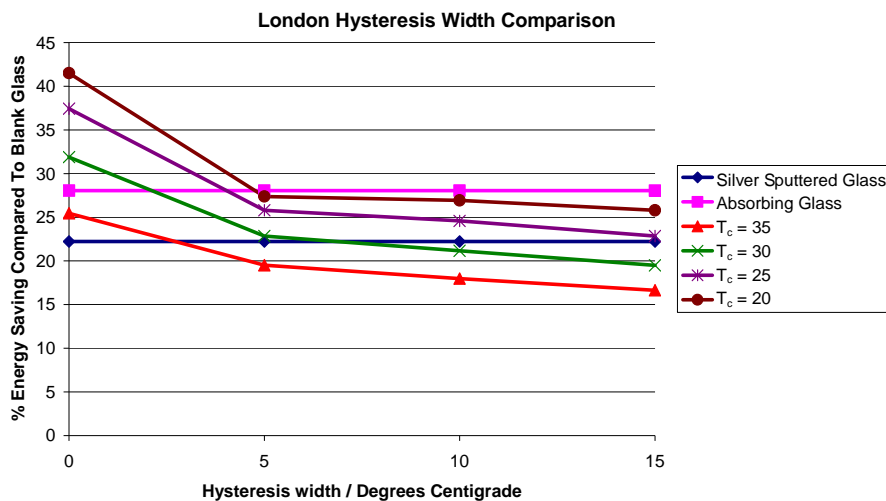
Figure 11. It shows the percentage energy saving of each system when compared to the blank glass system with variation of hysteresis width.
