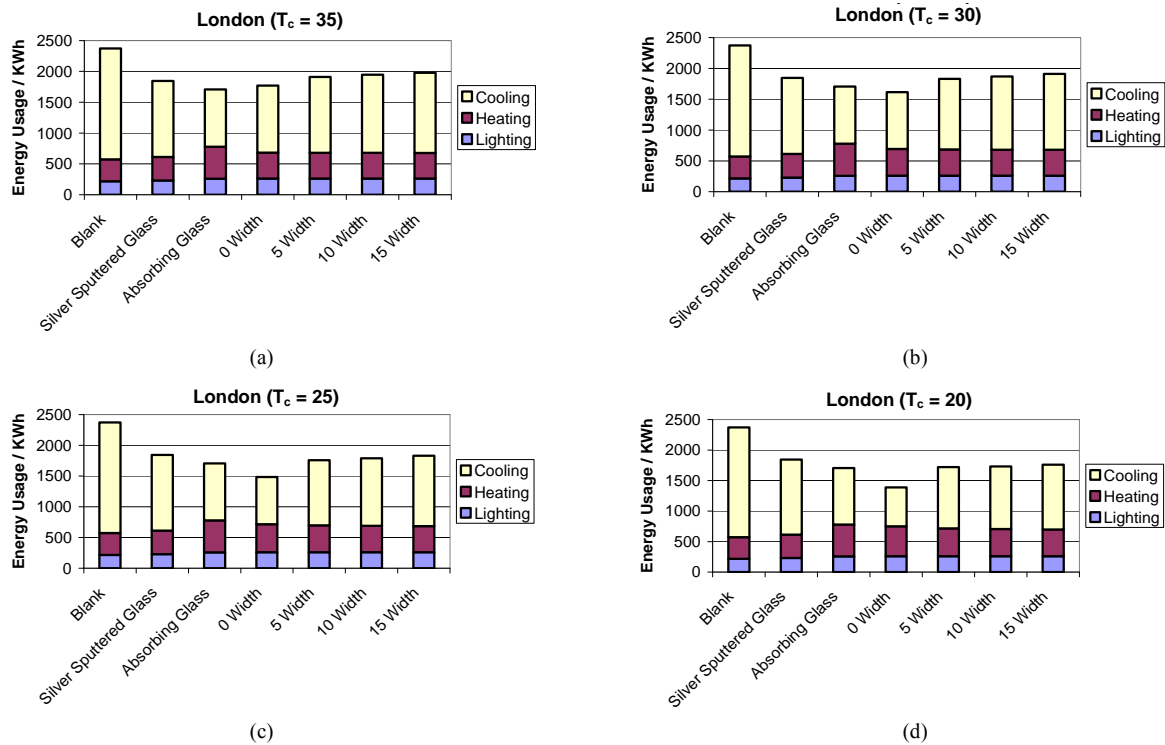
Figure 10. (a)-(d) show the breakdown of energy usage in a commercial building model based in London for varying values of T_c ((a) = 35°C, (b) = 30°C, (c) = 25°C, (d) = 20°C) and varying hysteresis width (0°C, 5°C, 10°C, 15°C). Each graph shows all modelled glazing systems. The colours correspond to the different energy requirements; yellow = cooling, maroon = heating, blue = lighting.
