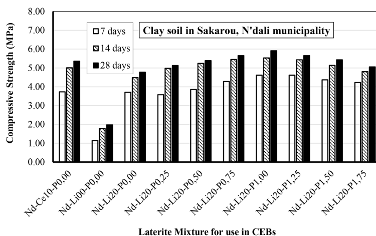
Figure 18. Compressive strengths of mortars (laterite + lime + PKC + water) prepared with lateritic soil from N'Dali municipality (Sakarou village).
