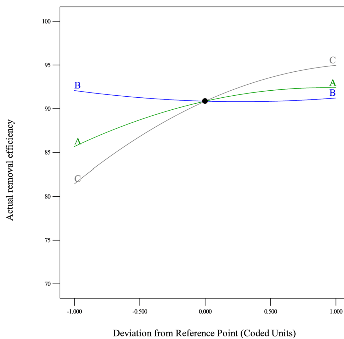
Figure 2. Perturbation plot of MB adsorption.
