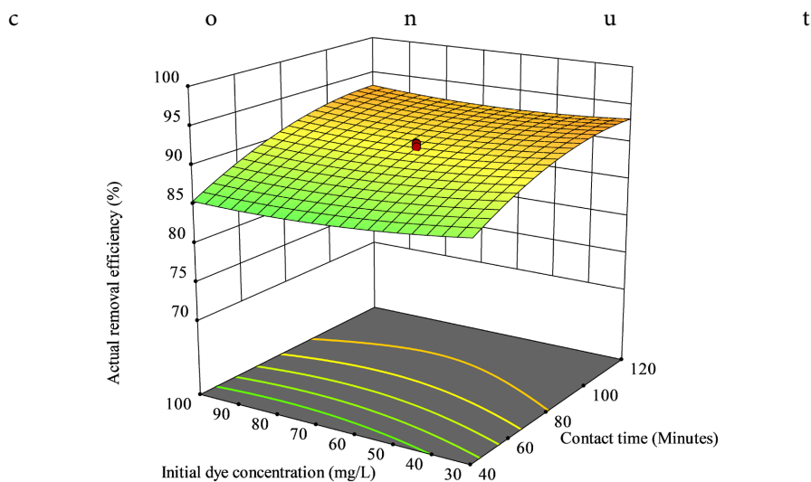
Figure 4. 3D-surface plot of the effect of initial dye concentration and contact time on MB removal efficiency (%) by coconut husk cellulose.
