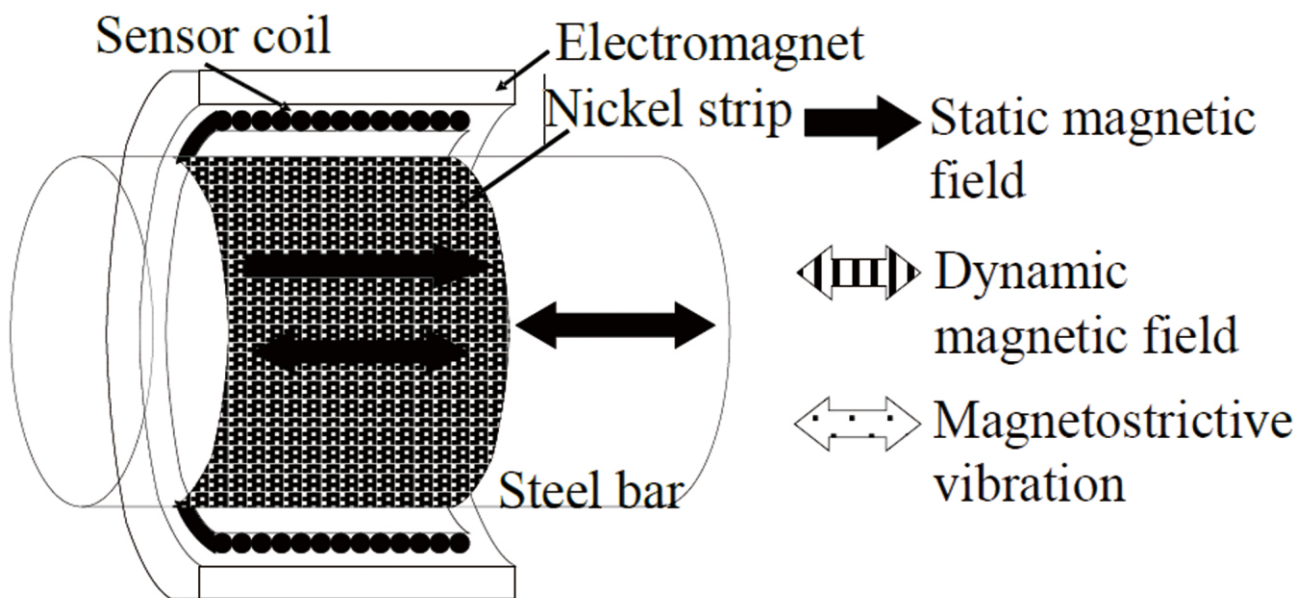
(C) Drive principle of a bar wave sensor using thin Nickel sheet
