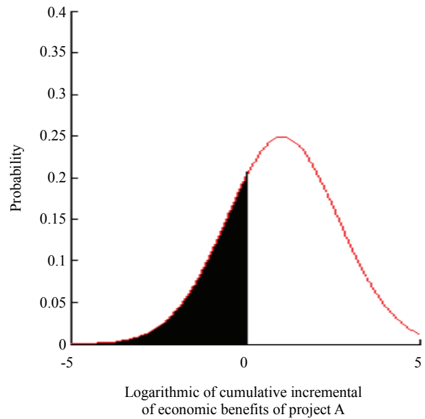
Figure 1. Normal distribution of project A
