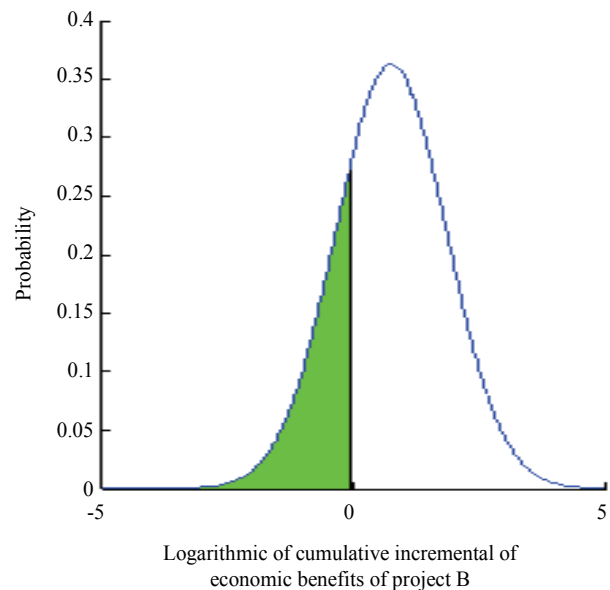
Figure 2. Normal distribution of project B
