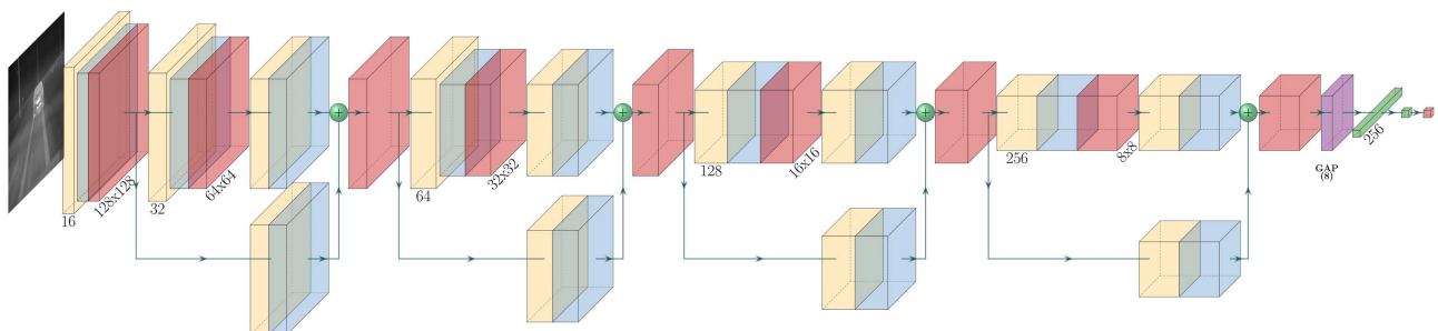
Figure 7. ResNet based trailing distance model architecture.
