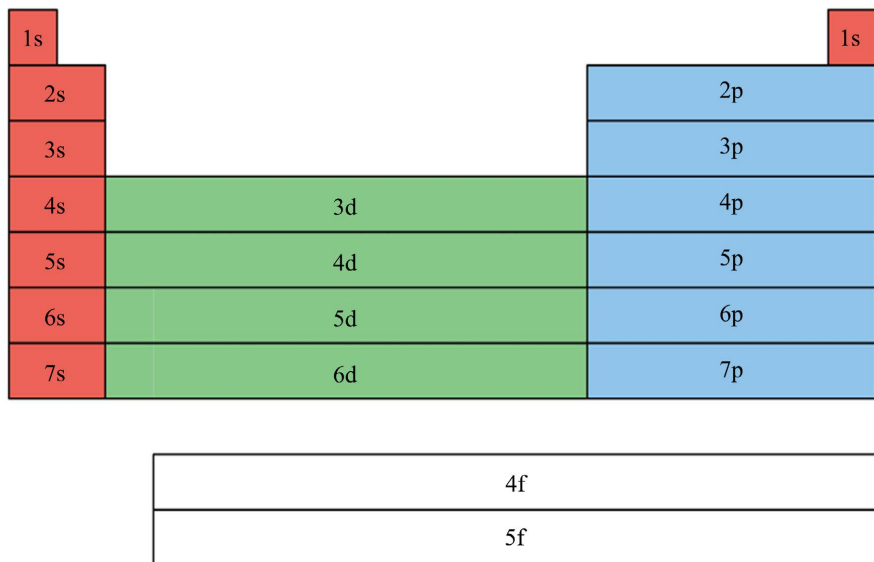
Figure 26. External electron orbit in Mendeleev's Periodic Table.
