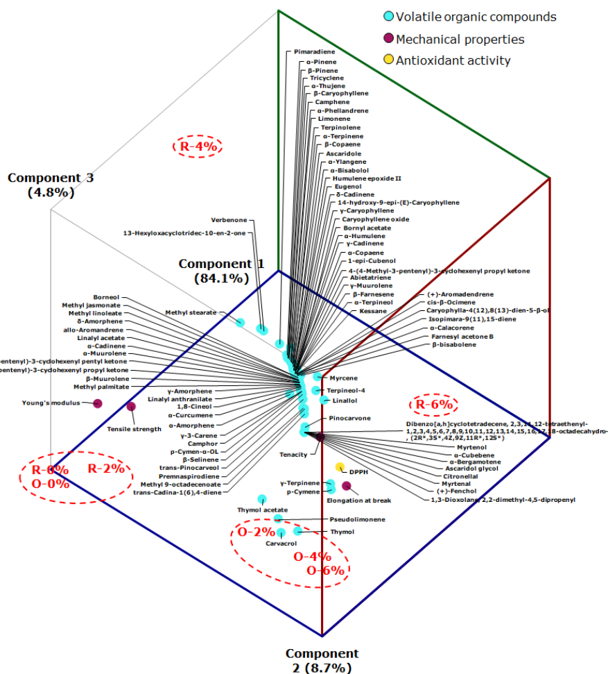
Figure 4. Tridimensional biplot from films with types (O = Oregano, R = Rosemary) and levels (0%, 2%, 4%, and 6%) of essential oil (scores) versus volatile organic compounds, mechanical properties, and antioxidant activity (loadings) in relation to the principal components.
