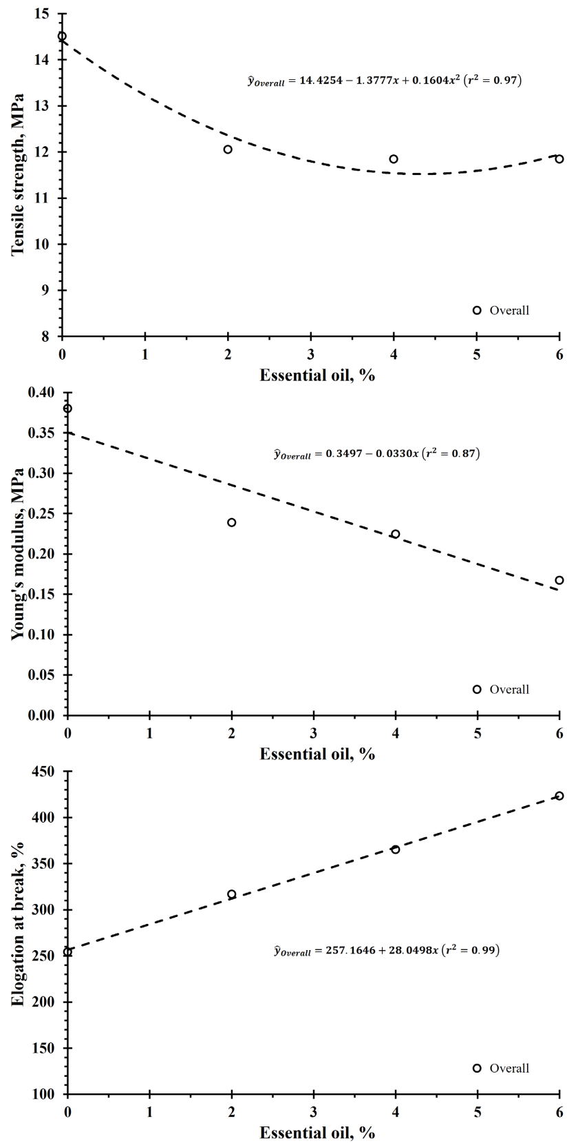
Figure 2. Mechanical properties of collagen fiber and polyvinyl alcohol films with different types and levels of essential oil.
